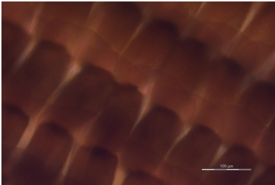
True color of Blue Morpho butterfly wing
