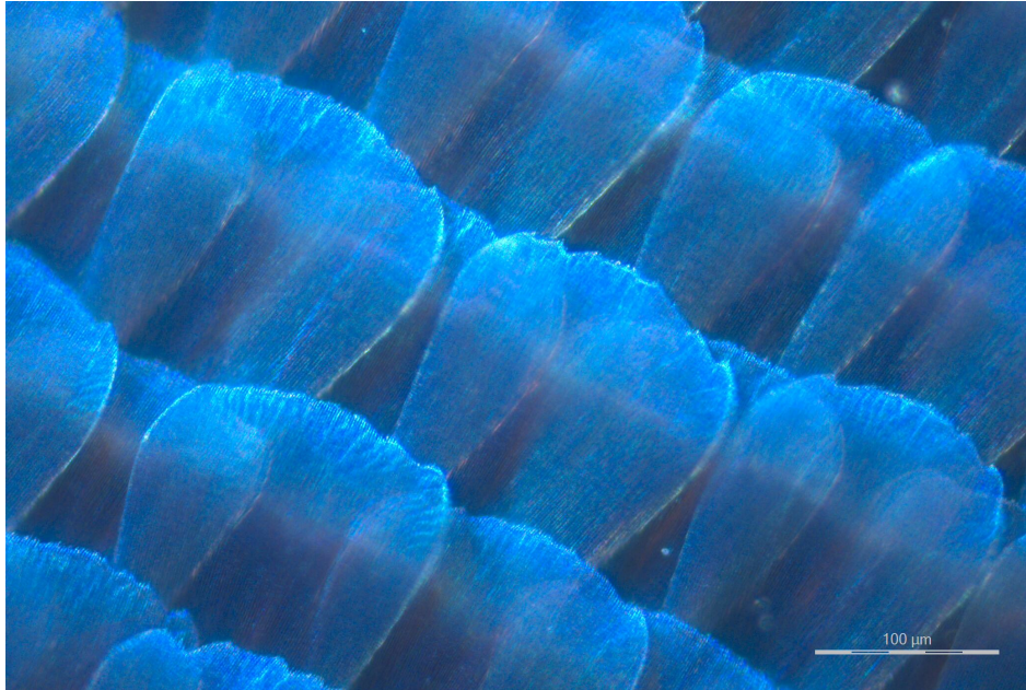
Light reflecting off Blue Morpho butterfly wing
