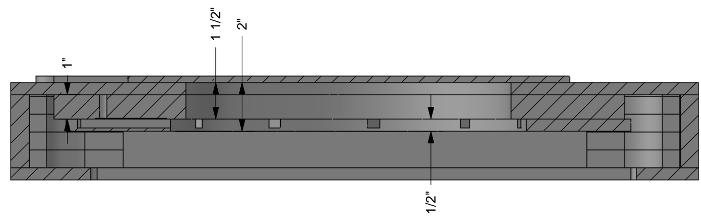
SECTION L-L SCALE 1 : 4
